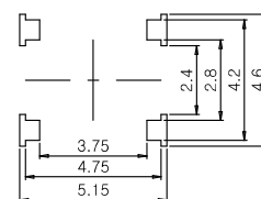
PCB Dimension
